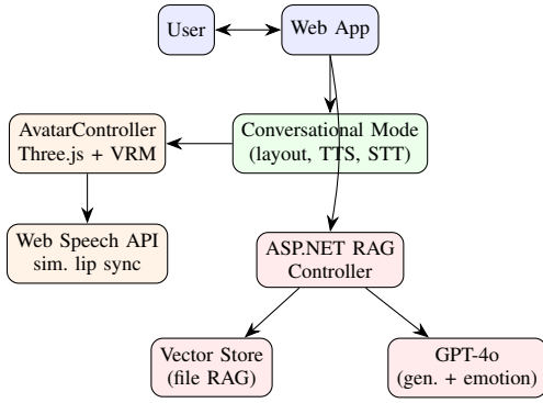
Figure 2. Ariel architecture. The RAG/LLM back end is shared by both conditions; the toggle enables or disables embodiment, voice and the avatar.
